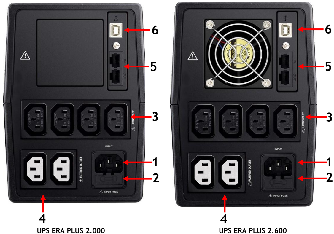
Figure 2 - Rear Side
